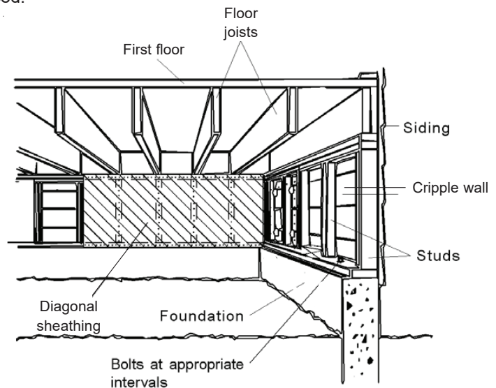
Figure 16 - Diagonal Sheathing. Common in older homes.
