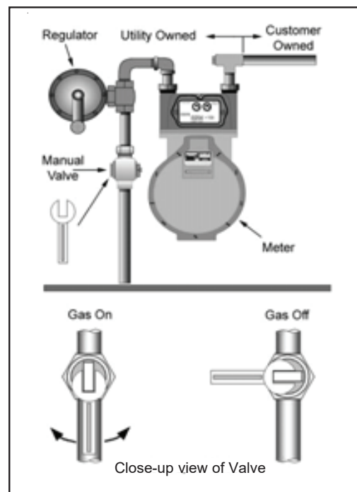
Figure 36—Manual Shutoff Valve Location
